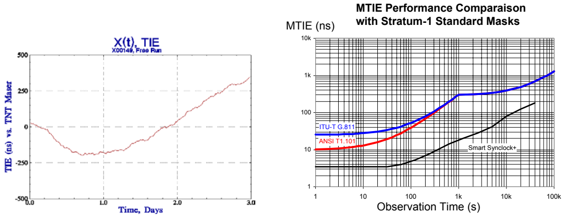
Figure 7a,b – Smart SyncClock+® Holdover Performance vs. Stratum-1 Standard Masks
