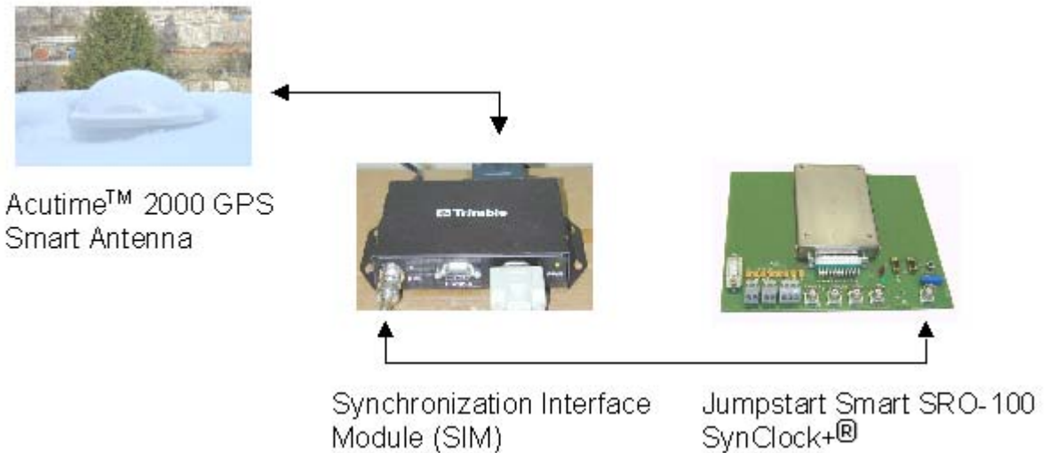
Figure 1 – Interconnection Setup
